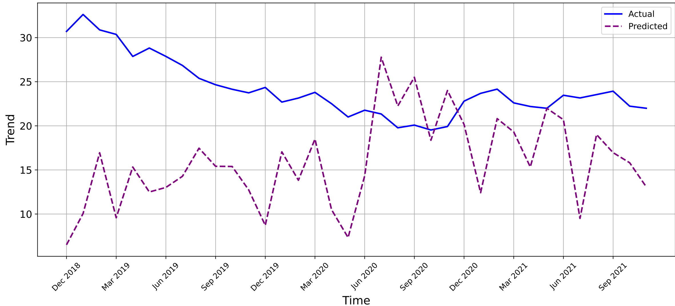
Solution_Bayesian Network_Mentions - Validation
